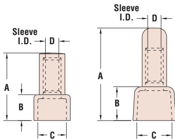
Part No. 2988** Features Extra Clearance Beyond Sleeve.
