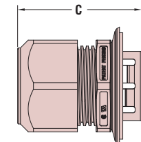
SEALING FLANGE/ WASHER CONSTRUCTION
